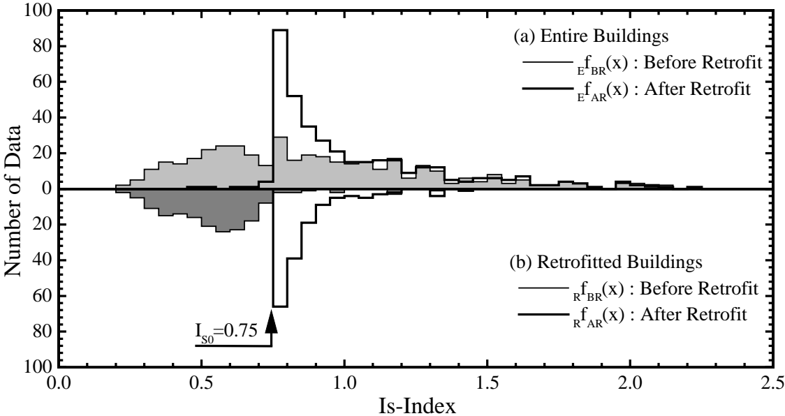
Figure 5. Distribution of Is index in the first story
