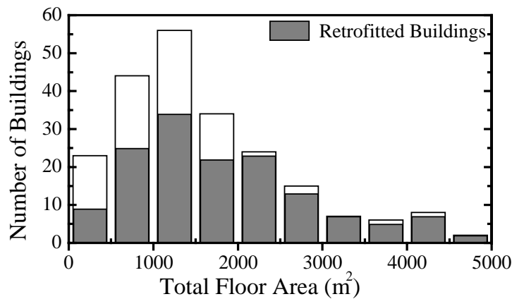
Note: Shaded areas denote retrofitted buildings. Figure 4. Basic statistics of 219 buildings investigated
