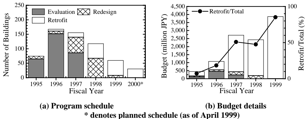
Figure 3. Outline of seismic retrofit program of school buildings constructed before 1981 in Ota City
