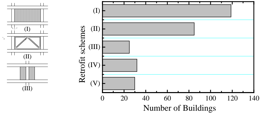
Figure 8. Employed retrofit schemes
