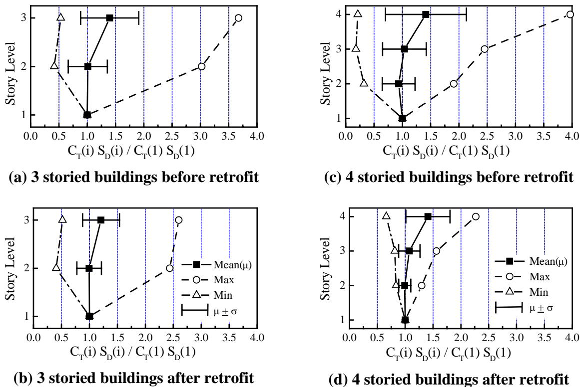
Figure 9. Distribution of lateral strength ratio R_s(i) ( = C_T(i) \times S_D(i) / C_T(1) \times S_D(1) ) along stories
