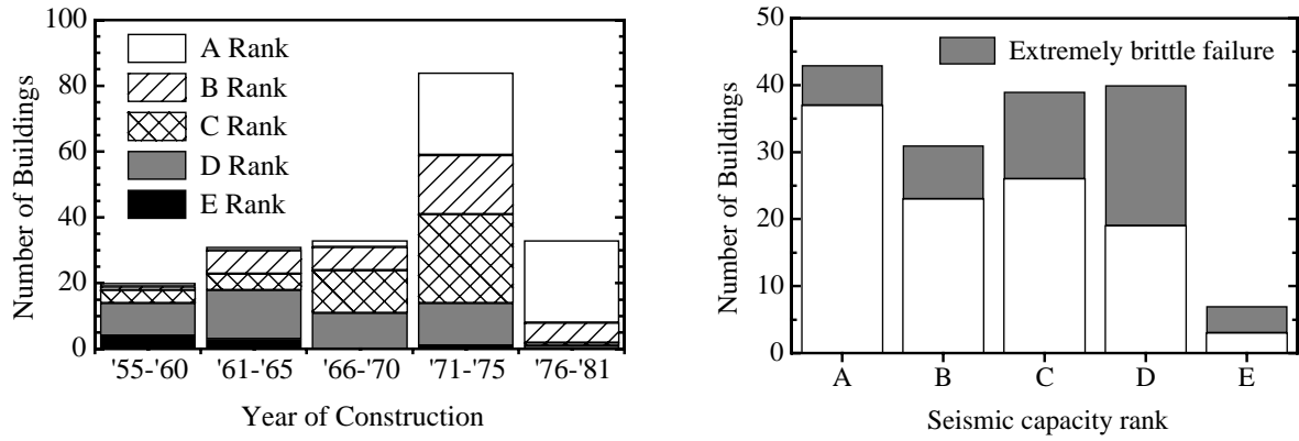
(a) Distribution of seismic capacity ranks (b) Ratio of buildings with brittle failure Figure 6. Seismic capacity ranks and ratio of buildings with brittle failure
