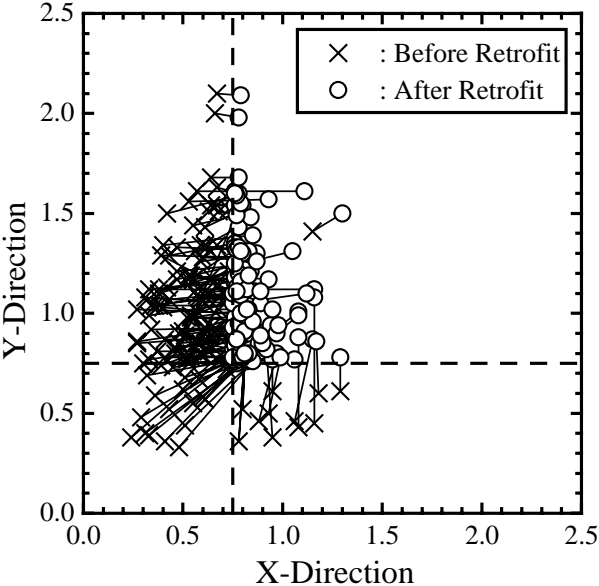
Figure 7. Correlation of I_s index in the first story before and after retrofit
