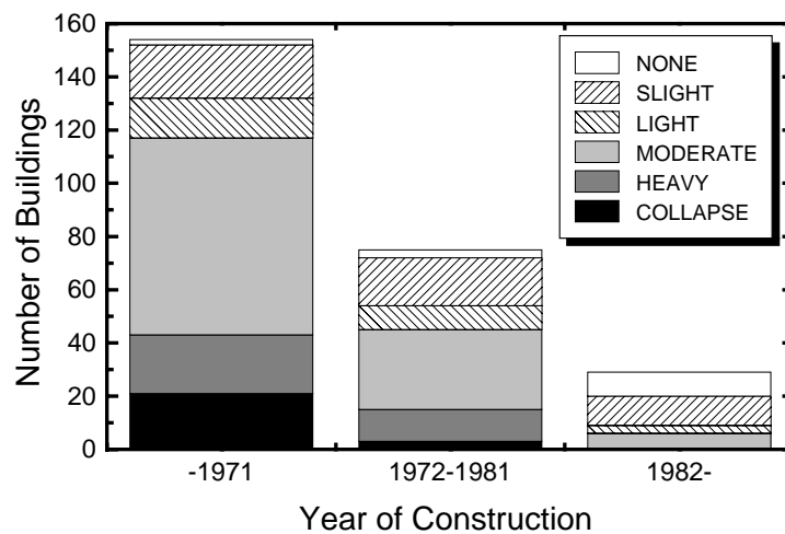
Figure 2. Damage statistics of RC school buildings during the 1995 Kobe Earthquake
