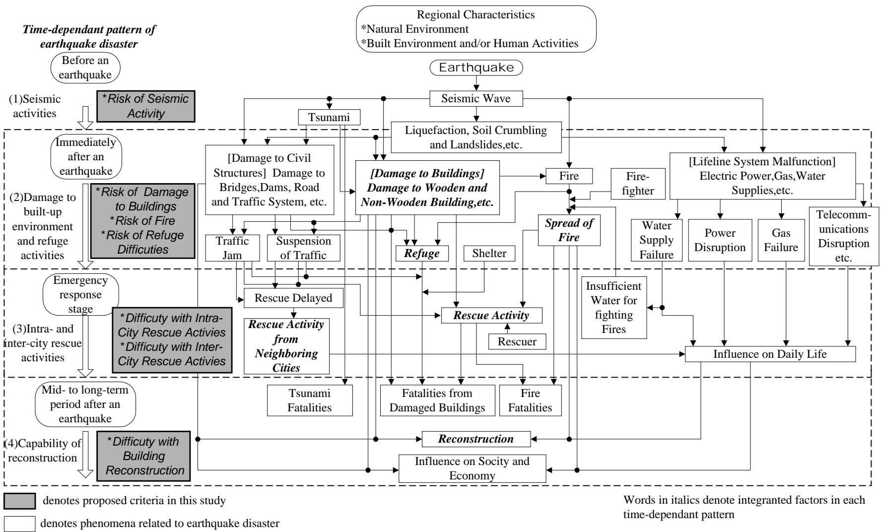
Fig. 1 Relationship between an earthquake disaster and interactive effects based on typical earthquakes experienced in Japan.
