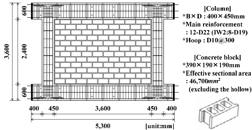
Figure 2. Details of specimen IW1
