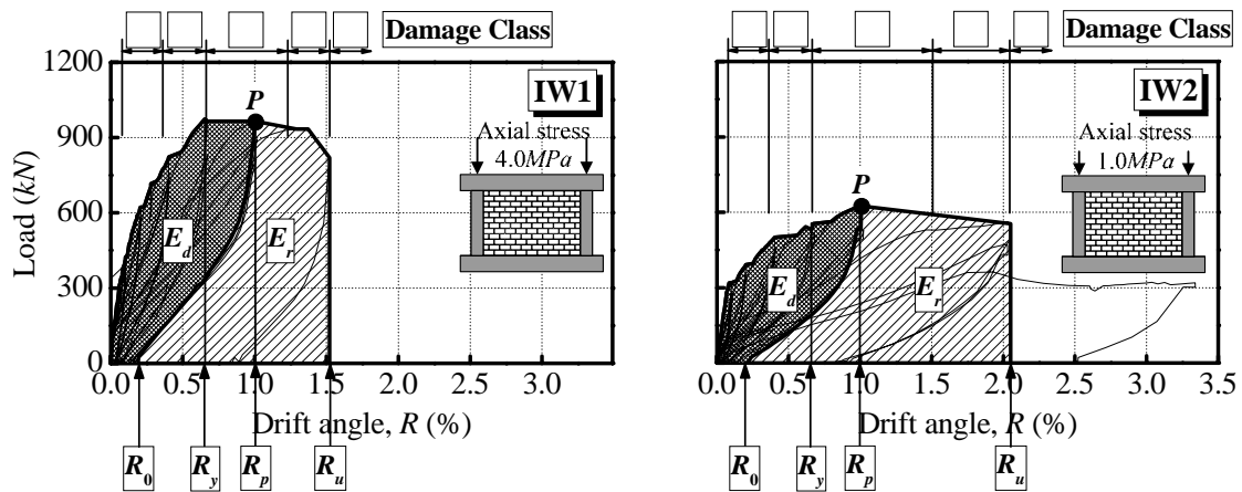
Figure 6. Load-drift angle relationship of specimens IW1 and IW2
