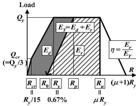
Figure 8. Simplified hysteretic model
