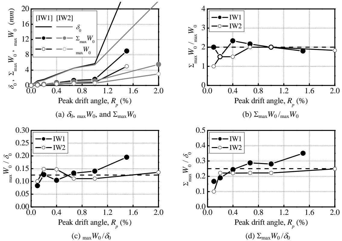
Figure 5. Relationship of residual crack width of CB wall \max W_0 , residual deformation of frame \delta_0 , and peak drift angle R_p
