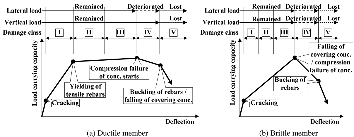
Figure 7. Schematic illustrations of damage class vs. load carrying capacity (JBDPA, 2001 and Nakano et al., 2004)
