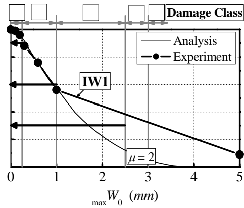
Figure 11. Seismic capacity reduction factor \eta vs. damage class
